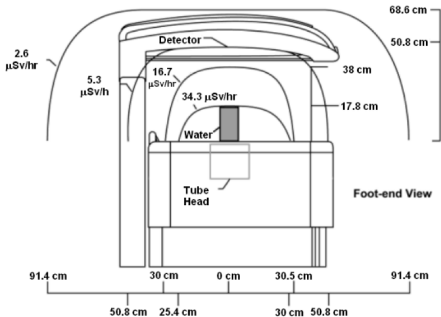
Isodose diagram: Foot-end view, Prodigy compact table
