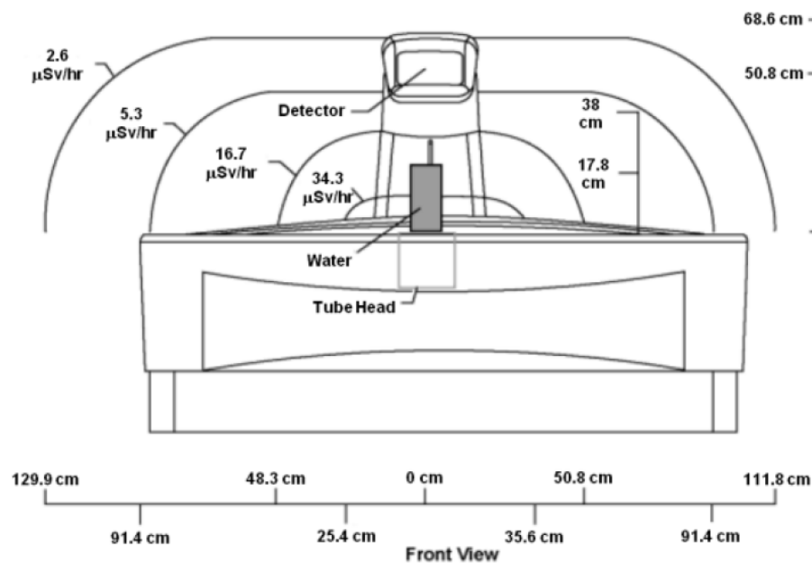
Isodose diagram: Front view, Prodigy compact table
